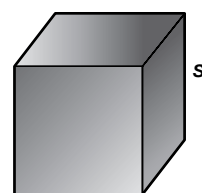
Surface area of a cube = 6s^2
